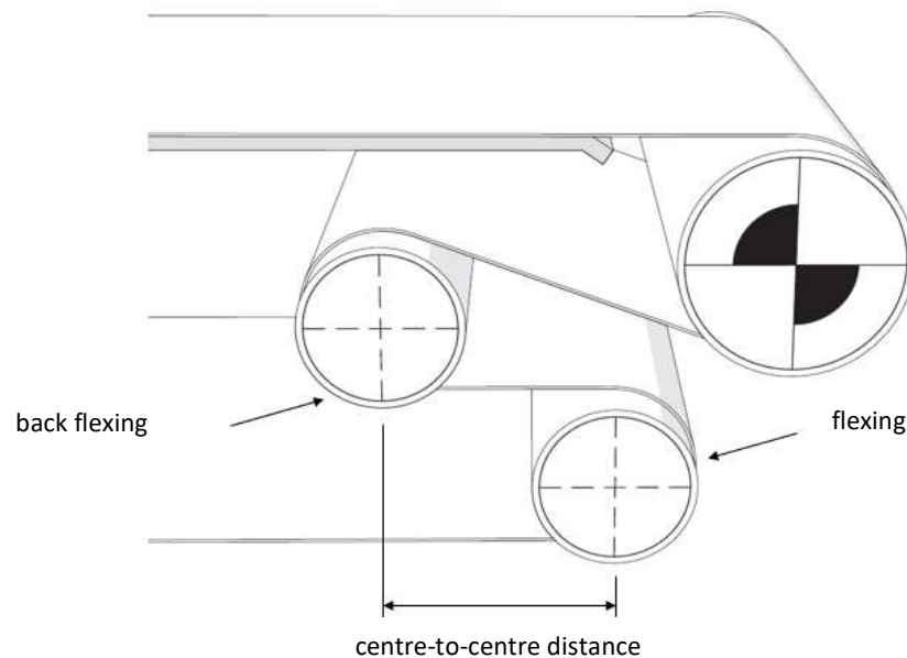
Image 27: centre-to-centre distance
