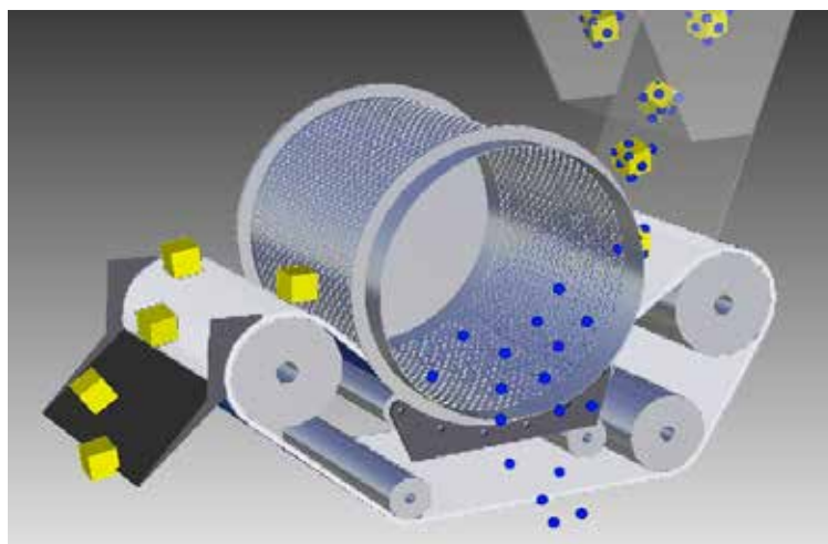
Diagram of the separating process
