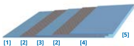
具有双面涂层和 Amseal 封边保护的双层输送带: [1] 底层; [2] 织物; [3] 内层; [4] 顶层; [5] Amseal 条带
