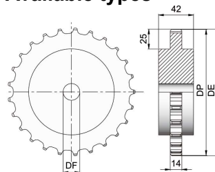
Drive - Idler Sprocket
